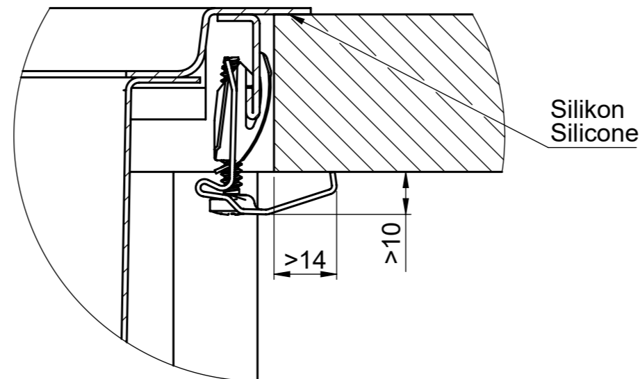
X (1:1)
