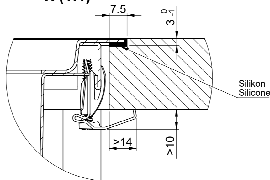
X (1:1)
