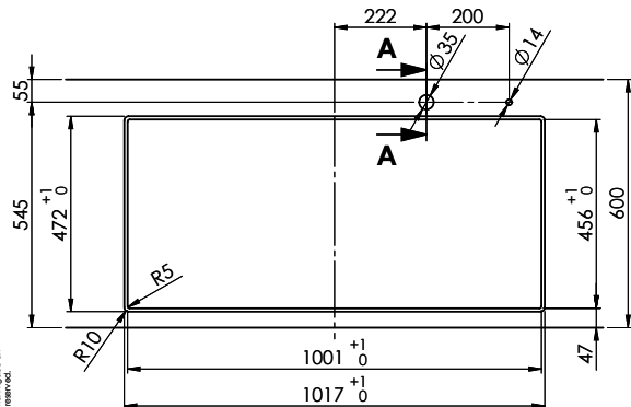
X (1:1)
